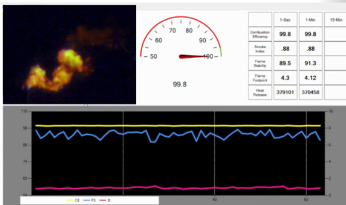
Mantis™ dashboard with live video feed (shown top-left)
